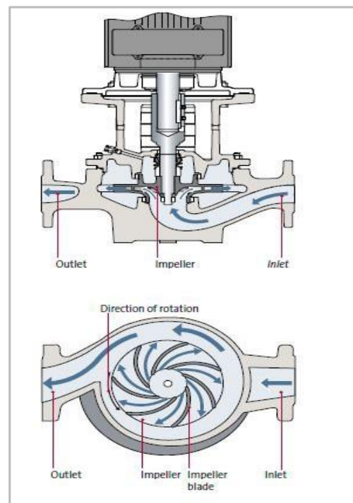
Centrifugal pump (Source: Grundfos).
