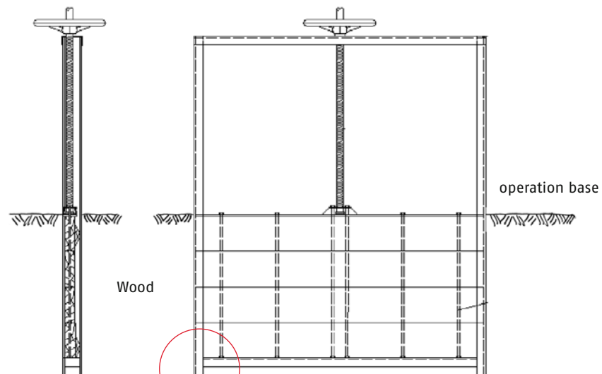
Sliding gate fitted with spindle
