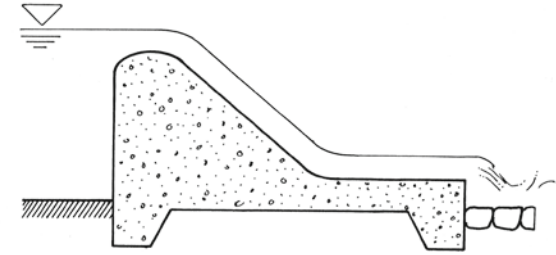
Concrete gravity weir
