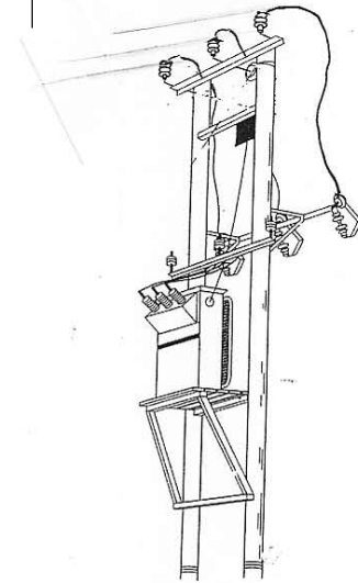
Pole-mounted MV/LV step-down transformer
