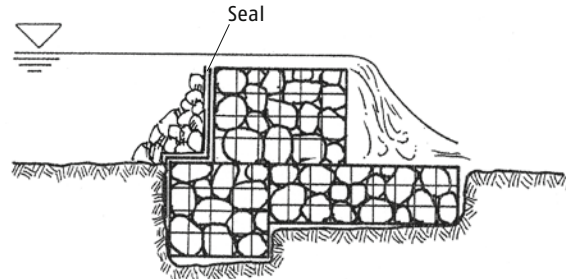
Gabion weir
